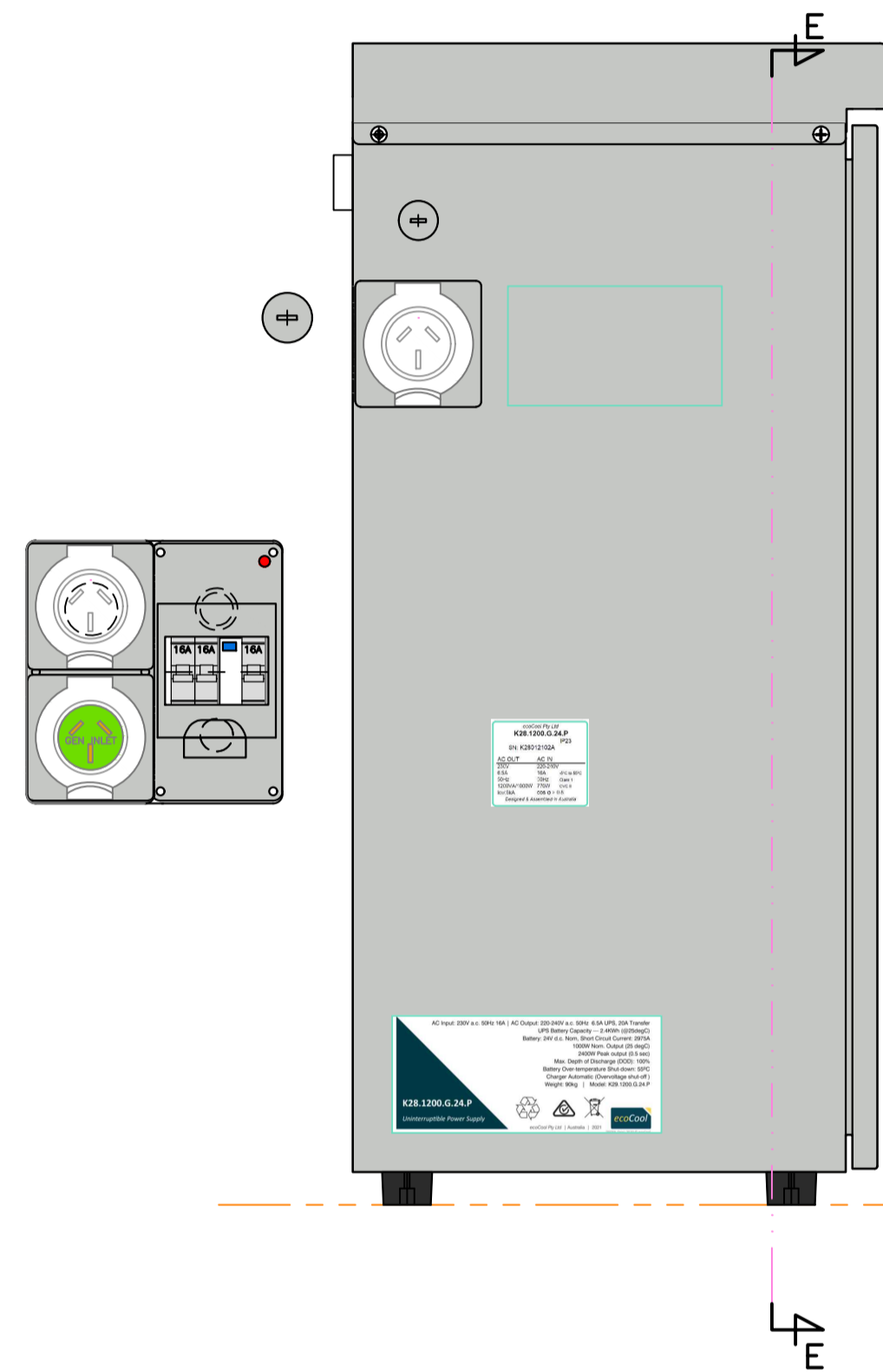
SIDE VIEW
